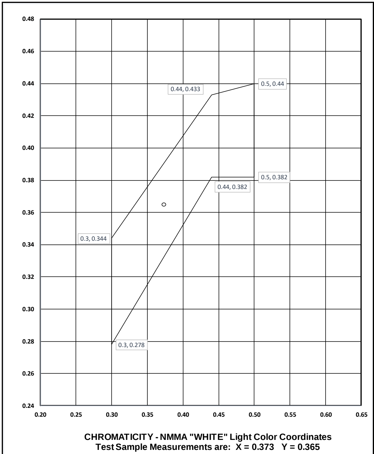
Figure 1: Chromaticity Plot of All-Round White Light / 2 mile
